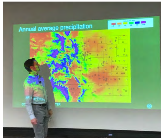
Colorado is not uniformly wet
