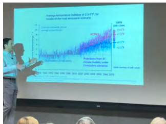
Historic rising temperatures
