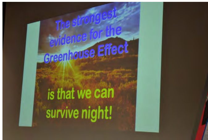
Without the Greenhouse Effect Temperatures would drop too low at night for life.
